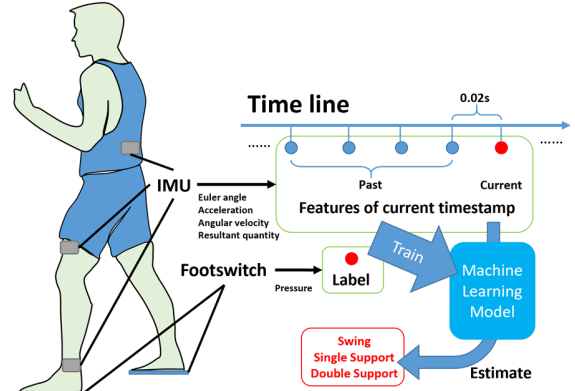
Fig. 1: System flowchart: IMU signals in combined with the calculated variables constitute the signals of one timestamp. Features of current timestamp are signals of current and four past timestamps. Current footswitch signal forms the label. Both features and labels are fed to the machine learning model.
